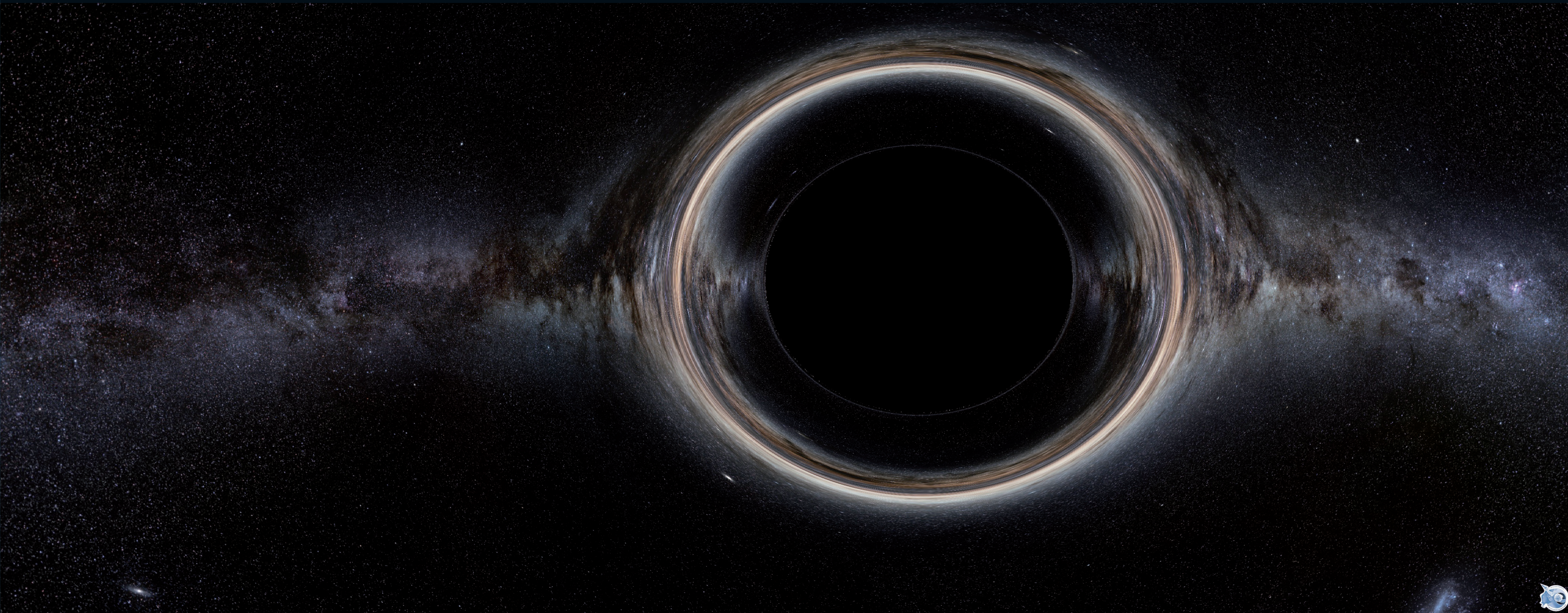
Visualisation of the Black Hole at the Centre of the Milky Way [visualisation: ESA Advanced Concepts Team (Alexander Wittig, Jai Grover) - [CC BY IGO] ; Milky Way background: ESO (S. Brunier) - [CC BY 4.0.]]
