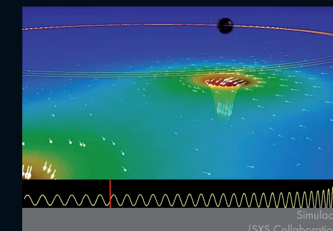
Simulacions (SXS Collaboration)
